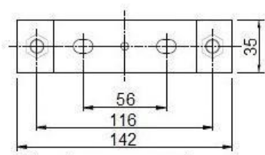
Hanging bracket dimension
